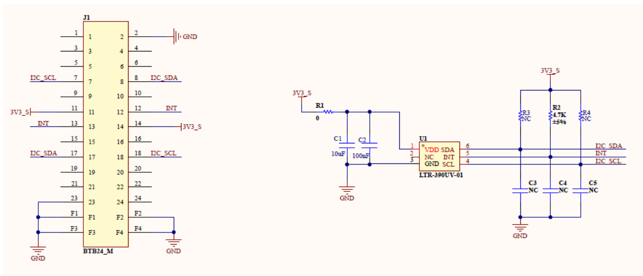
Figure 5: RAK12019 WisBlock UV Sensor Schematic Diagram
