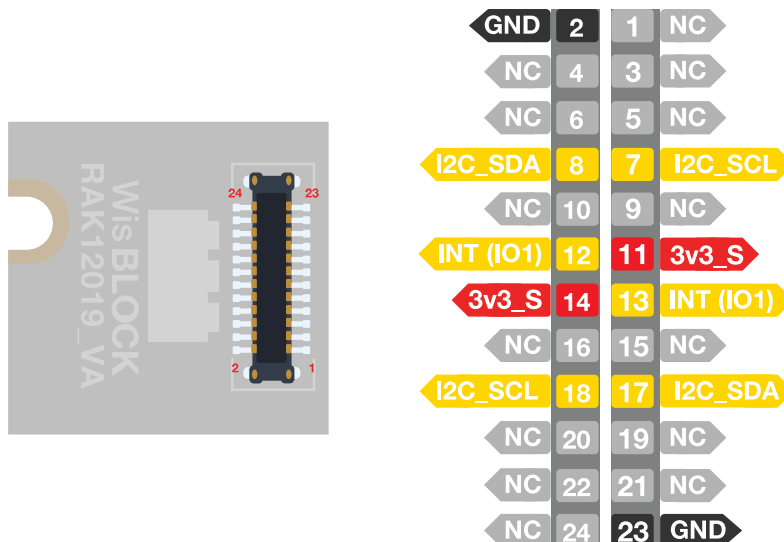
Figure 2: RAK12019 WisBlock UV Sensor Pinout
