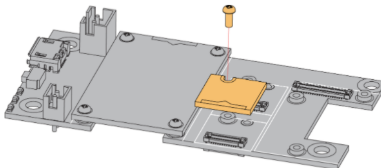
Figure 1: RAK12019 WisBlock UV Sensor Mounting
