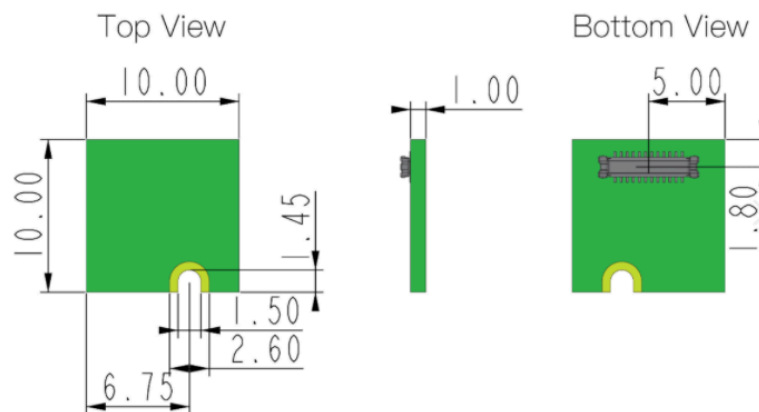
Figure 3: RAK12019 WisBlock UV Sensor Dimensions
